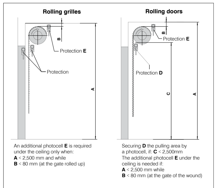
MINIMUM PROTECTION LEVELS OF THE MAIN CLOSING EDGE OF THE GATE ACCORDING TO PN-EN 12453:2017
